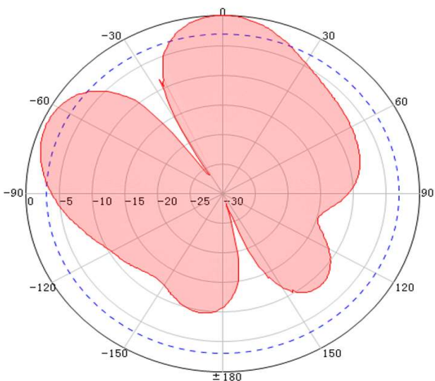
2100MHz Vertical
